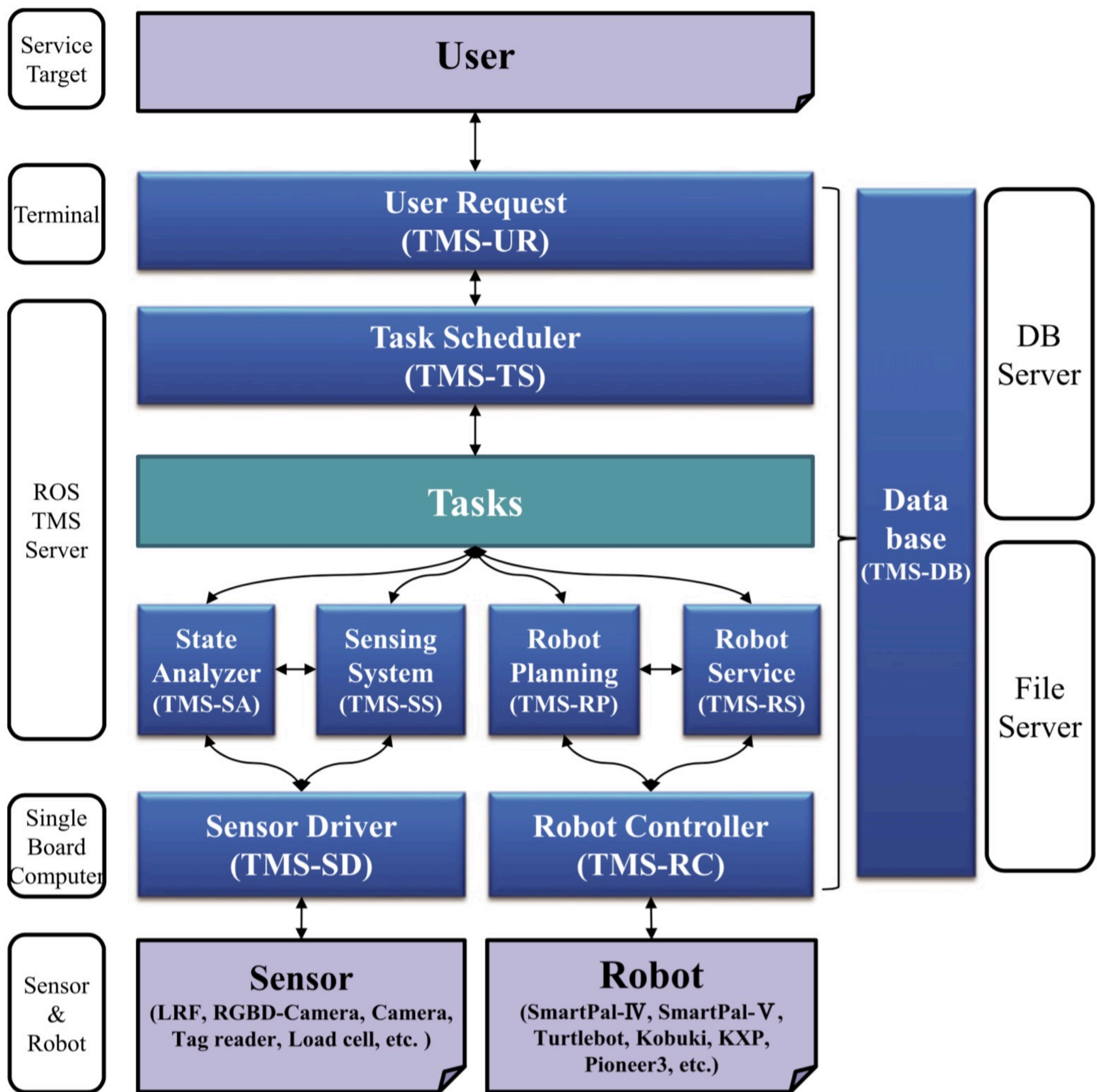
Fig. 4. Architecture of the ROS-TMS.
