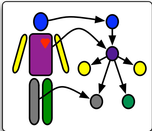
Scene Graph
