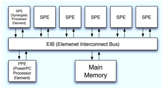
図 1 Cell Broadband Engine
