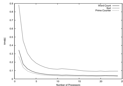
図 2 Execution time
