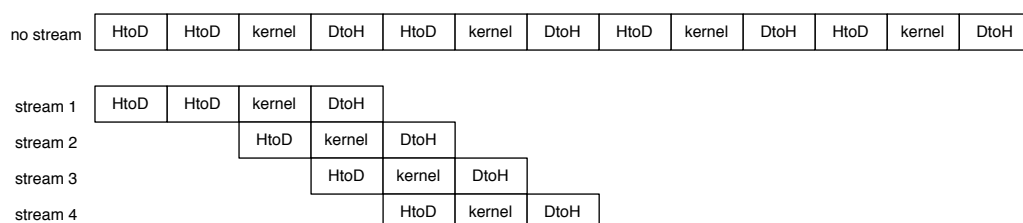
図 2.6: Parallel Execution
