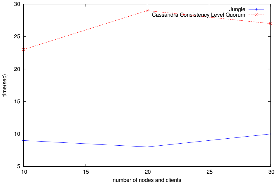
distributed read benchmark (Requests : clients * 50,000)
