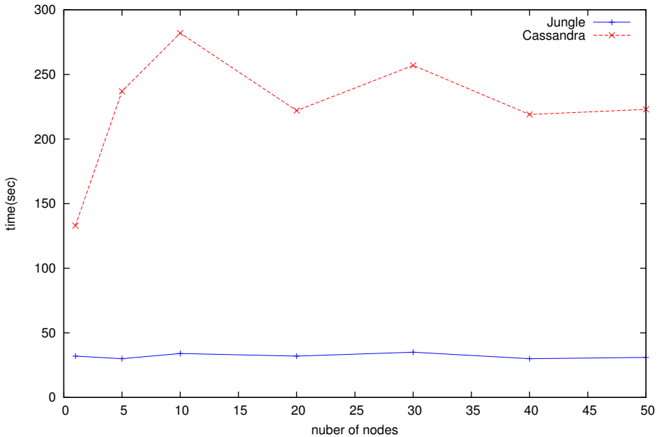
read benchmark
