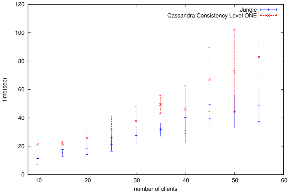
Single node read benchmark (Requests : clients * 20,000)
