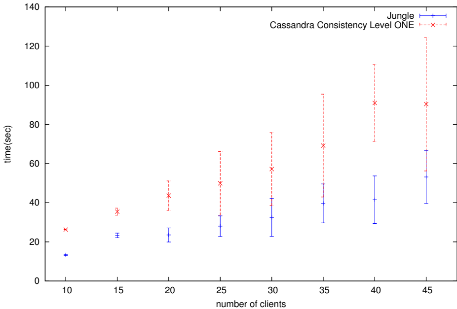
Single node write benchmark (Requests : clients * 20,000)
