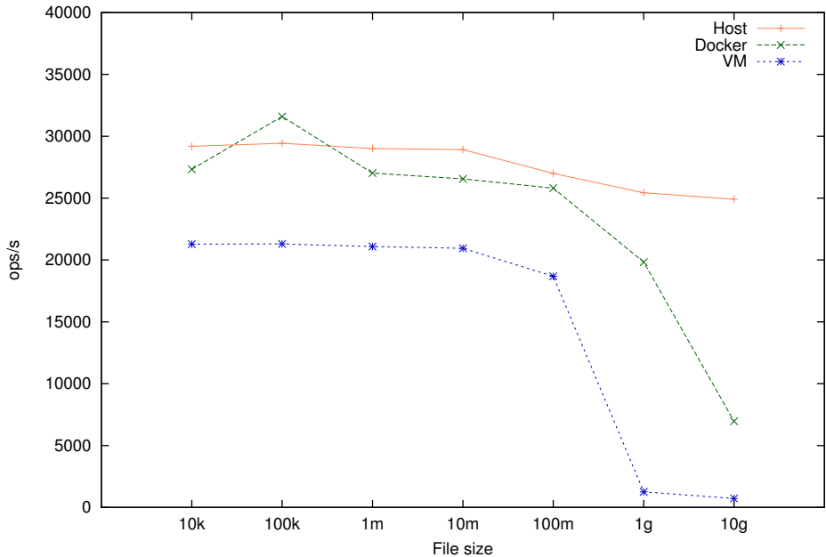
Filesystem write benchmark
