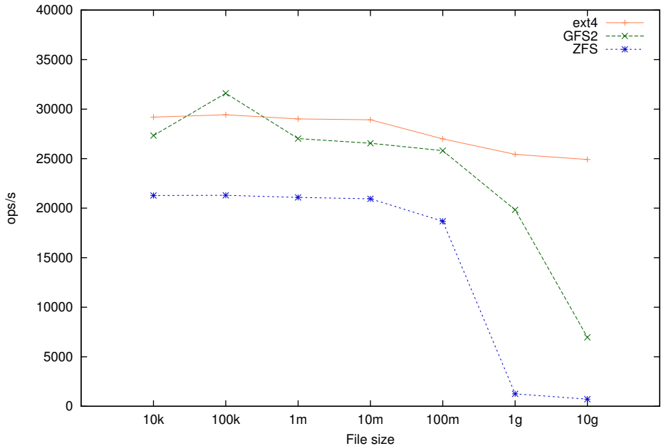
Filesystem benchmark benchmark
