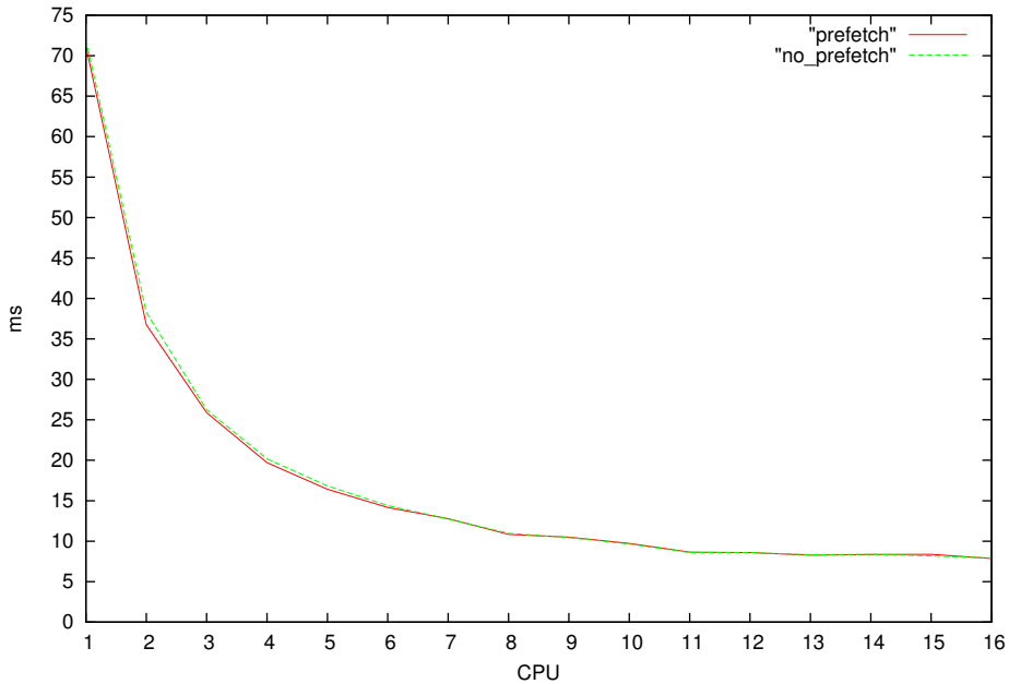
WordCount Benchmark
