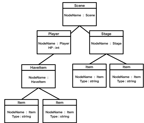
図2: GameTree
