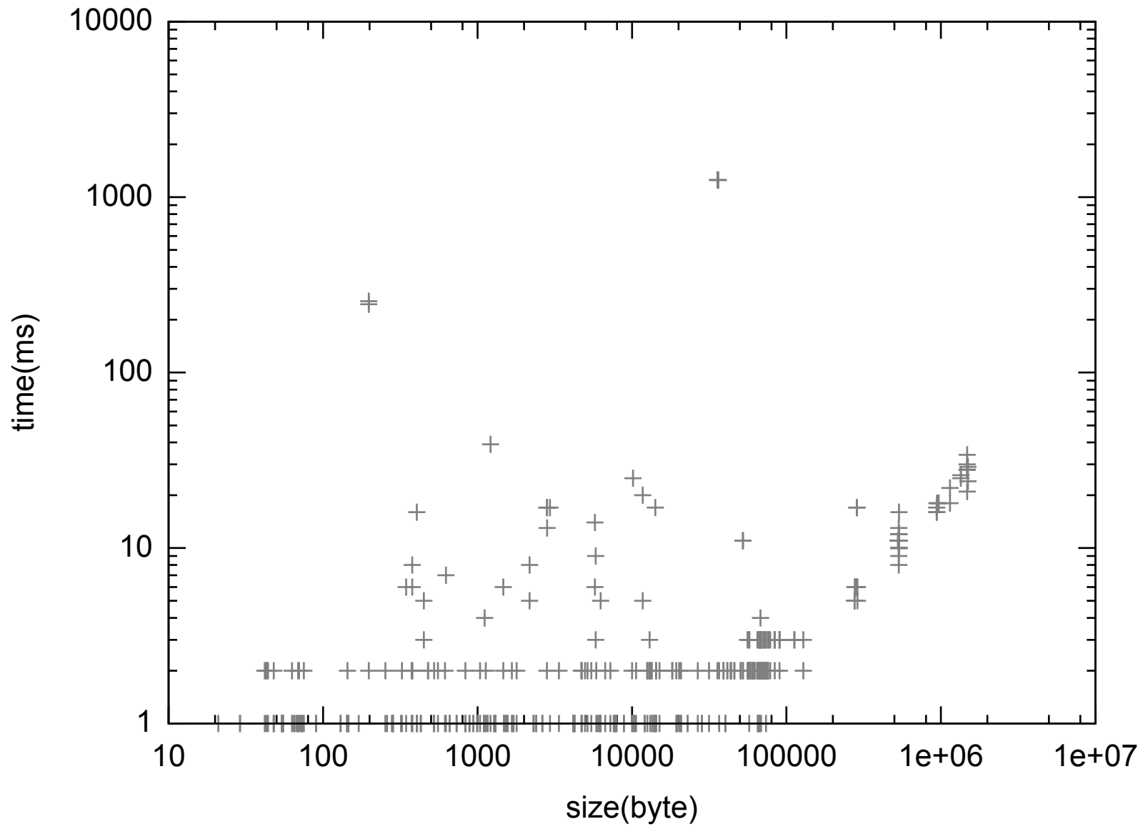
node depth1
