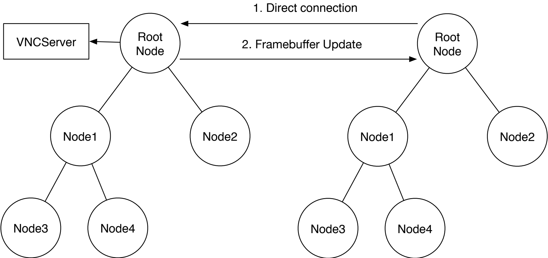
Tree VNC 1 (network1)
