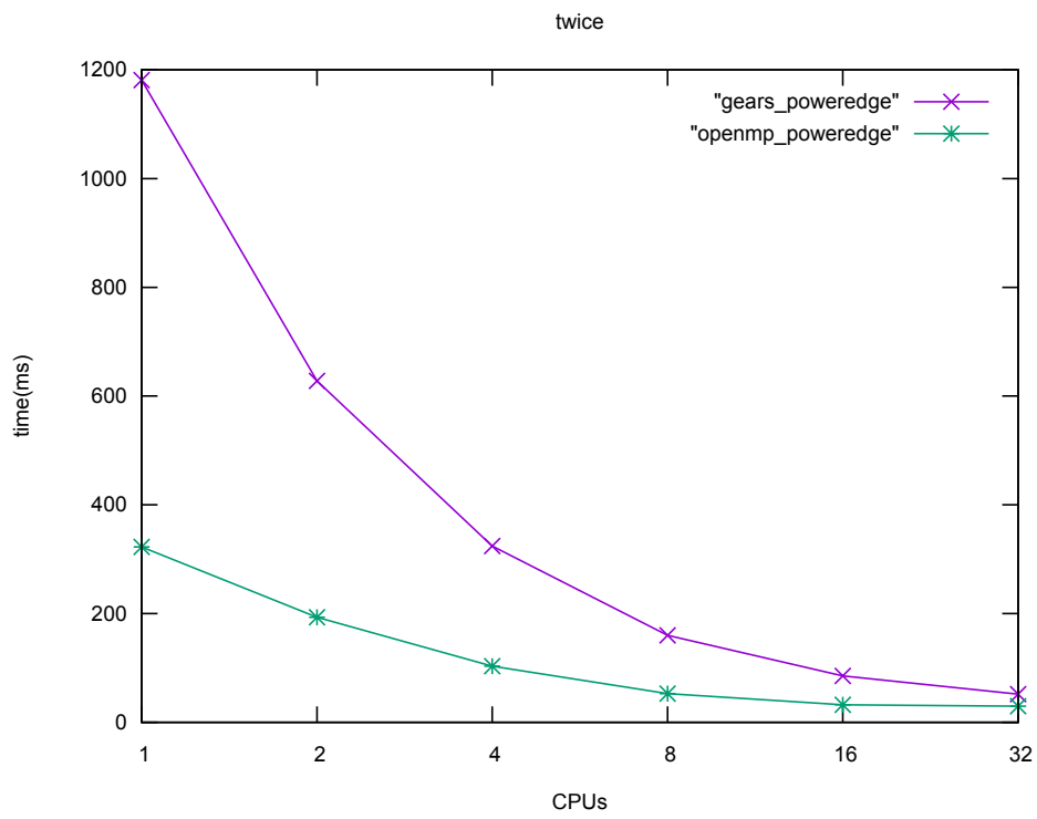
図 6.4: vs OpenMP
