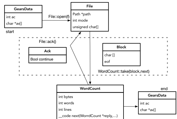
図 5: WordCount with Gearbox
